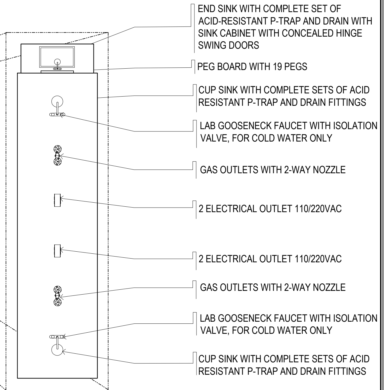
TYPICAL LABORATORY TABLE BLOW UP PLAN SCALE 1:30 MTS
