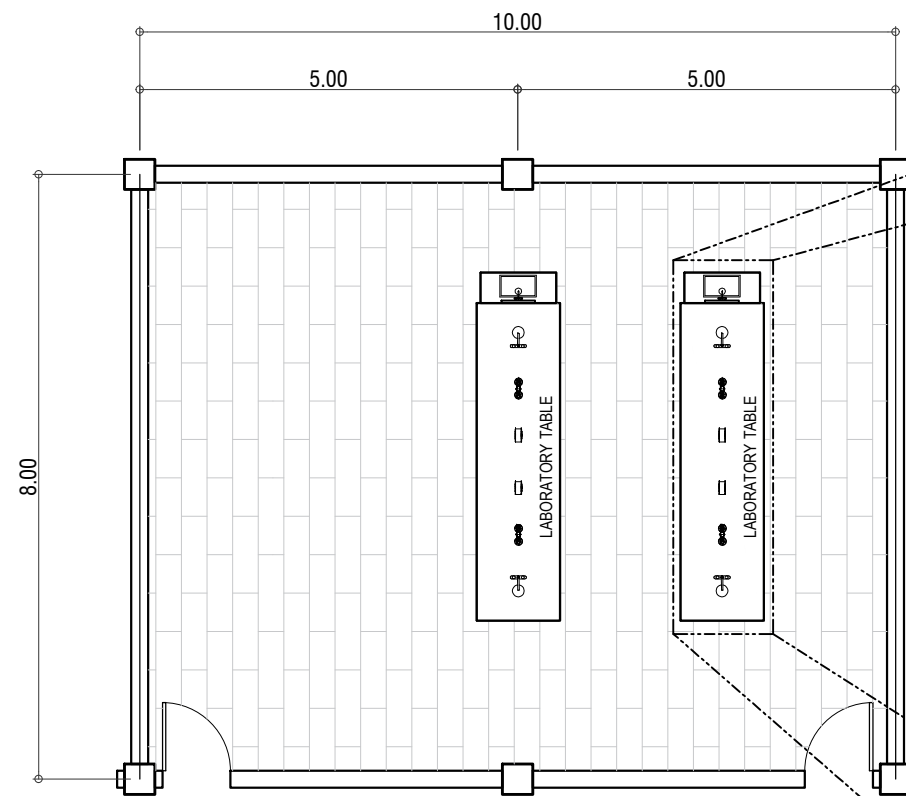
L.S 8 FLOOR PLAN SCALE 1:100 MTS
